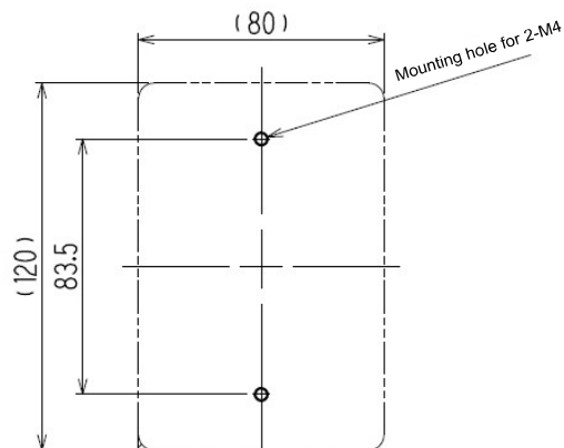
Installation dimension drawing (Installation board not used) Compatible with JIS single switch box
