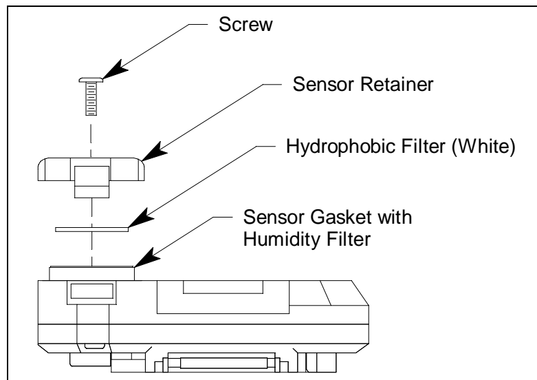
Figure 12: Replacing the Hydrophobic Filter
