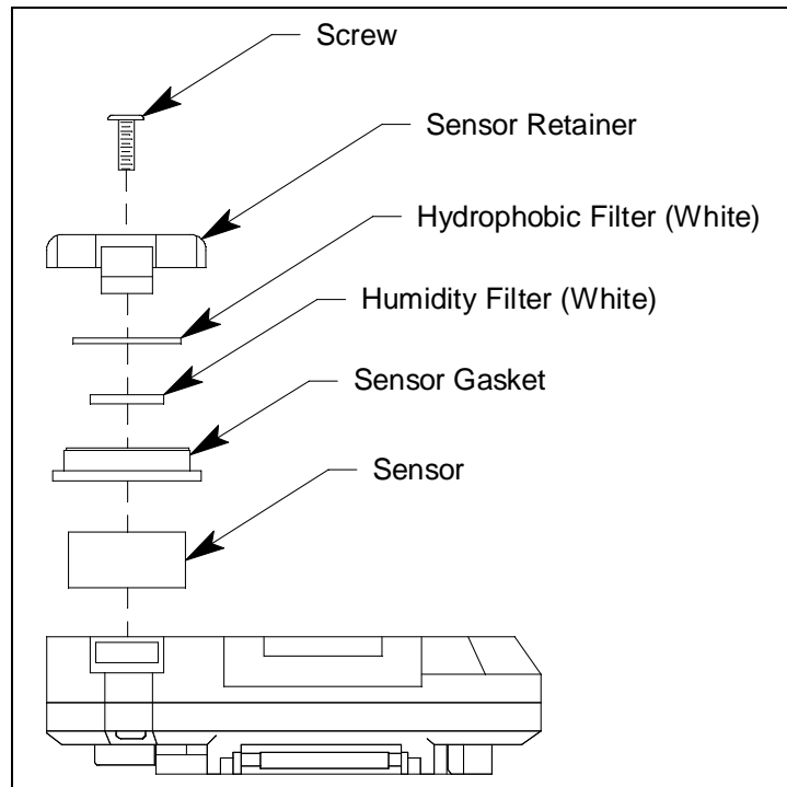
Figure 13: Replacing the Sensor
