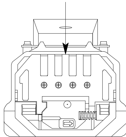
2. Push New Battery Pack Down
