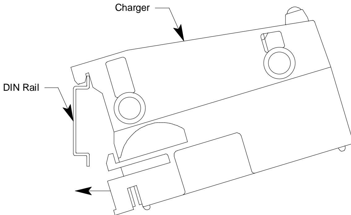
Figure 6: Installing a Charger on the DIN Rail
