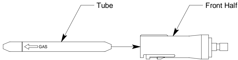
Figure 40: Inserting New Tube Into Front Half
