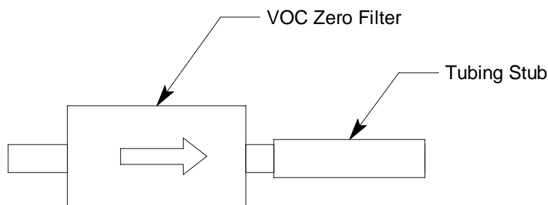
Figure 3: VOC Zero Filter
