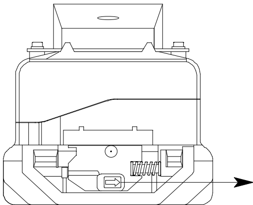
1. Be Sure Battery Pack Release Latch is Pushed to the Right
