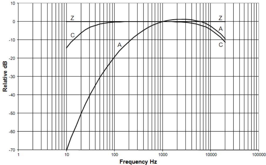
Figure B-5: All frequency weightings plotted together
