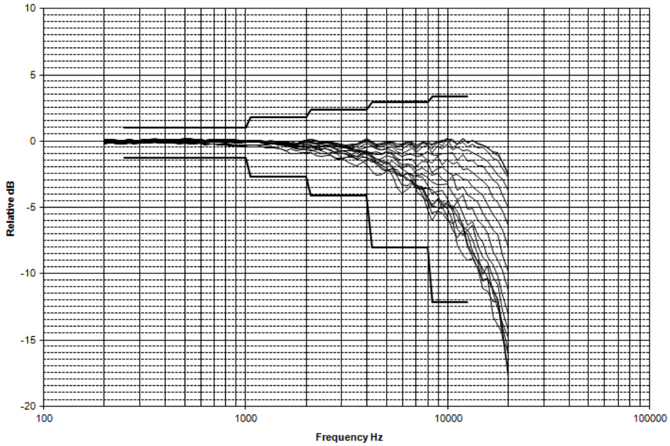
Directional frequency response positioned back-side toward noise source (0°-150° incidence angles)
