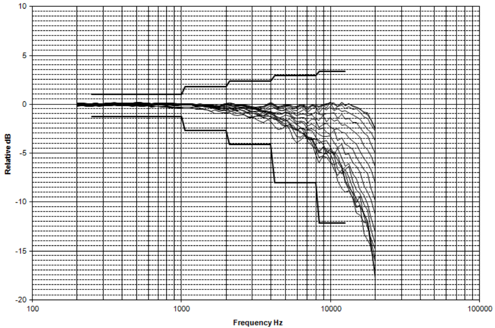
Directional frequency response positioned back toward noise source (0°-150° incidence angles)
