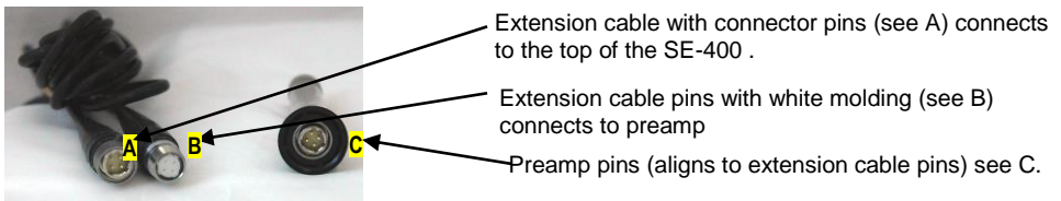
Figure 4-17: Example of extension cable and preamp
