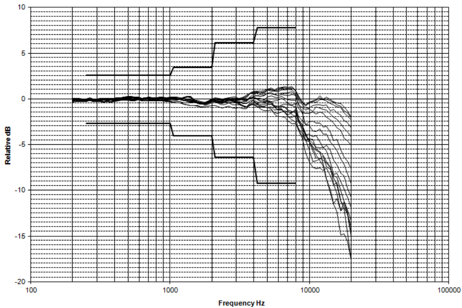
Directional frequency response positioned side toward noise source (0°-150° incidence angles)
