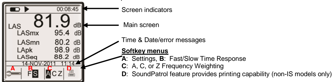
Figure 1-1: SE-400 Series Screen
