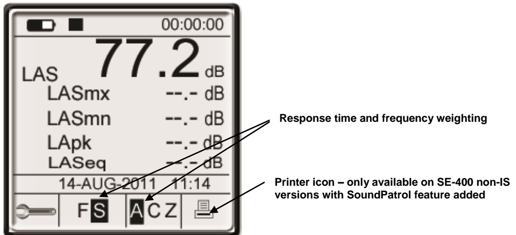
Figure 3-1: Response time and frequency weighting
