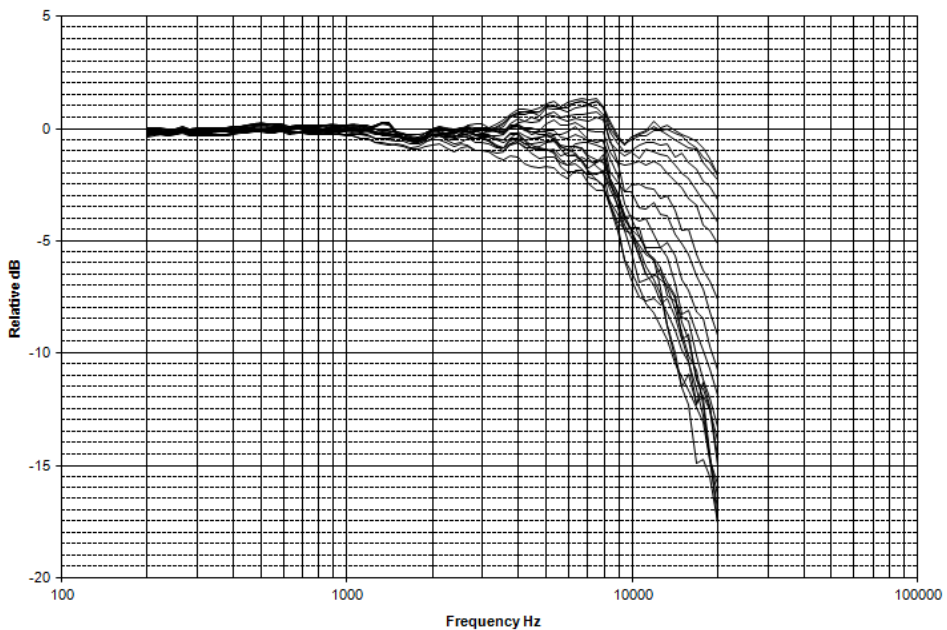
Directional frequency response positioned side toward noise source (0°-180° incidence angles)
