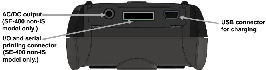
Figure 1-2: Connector and ports
