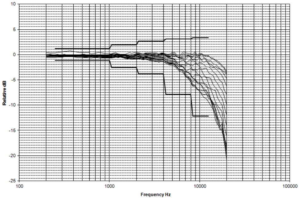
Directional frequency response using windscreen & remote preamp (0°-180° incidence angles)
