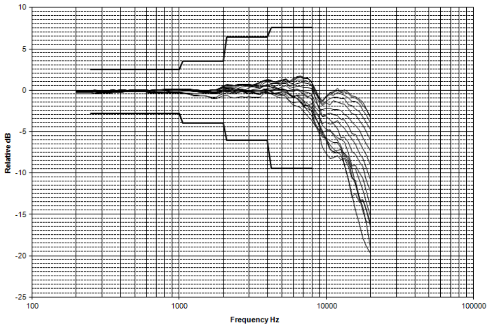
Directional frequency response positioned side noise source (0°-180° incidence angles)
