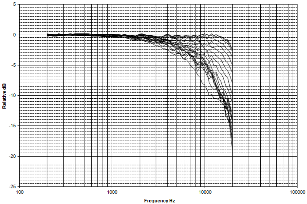
Directional frequency response positioned back-side toward noise source (0°-180° incidence angles)
