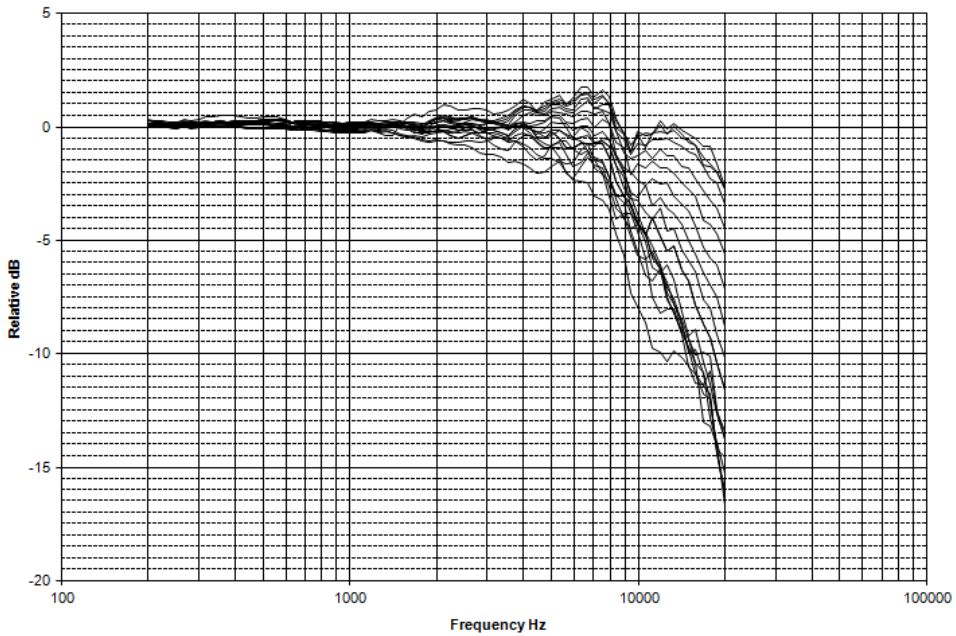
Directional frequency response facing back toward sound source (0°-180° incidence angles)
