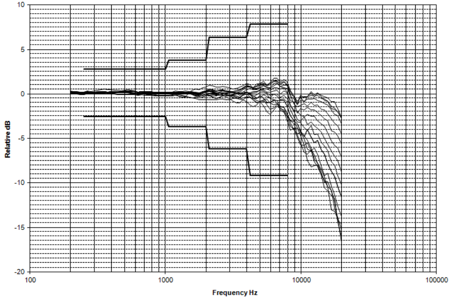
Directional frequency response facing back toward sound source (0°-150° incidence angles)
