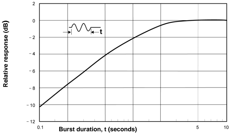
Figure B-2: Slow response to a tone burst
