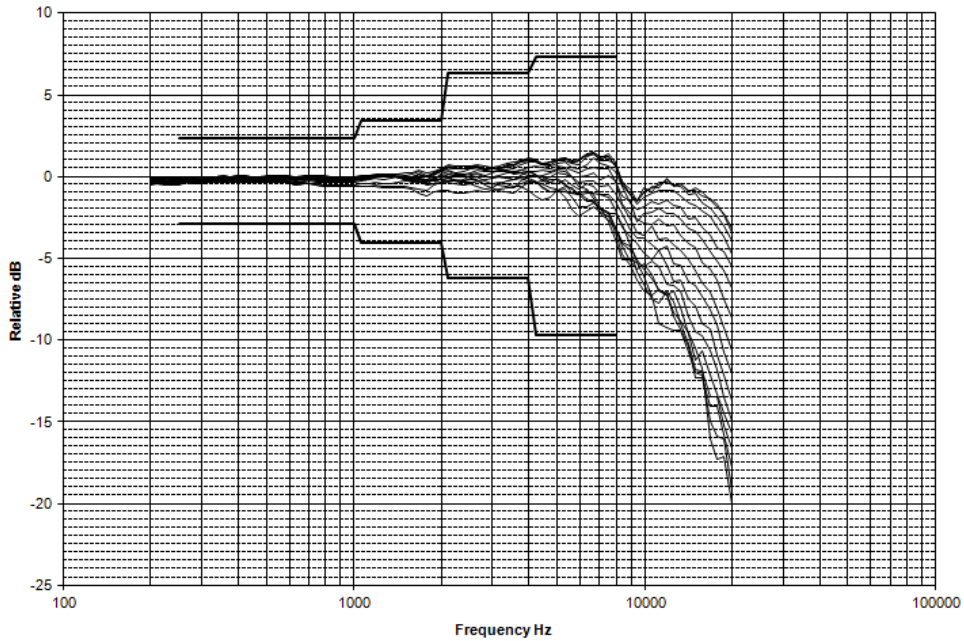
Directional frequency response positioned facing toward noise source (0°-150° incidence angles)
