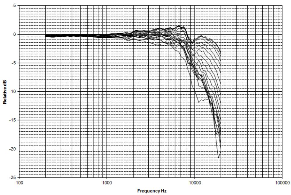
Directional frequency response positioned facing toward noise source (0°-180° incidence angles)
