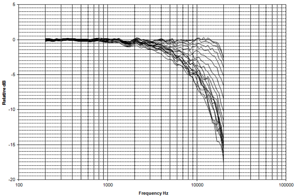
Directional frequency response positioned using side toward noise source (0°-180° incidence angles)
