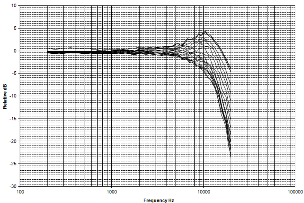
Directional frequency response positioned toward noise source (0°-180° incidence angles)
