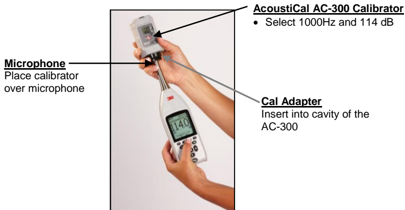
Figure 4-1: SE-400 Series and calibrating
