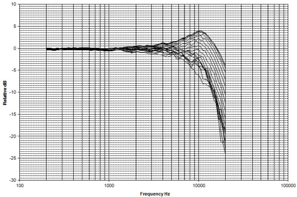
Directional frequency response positioned back toward noise source (0°-180° incidence angles)
